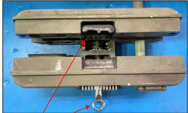
Burned Smart Fault Indicator
