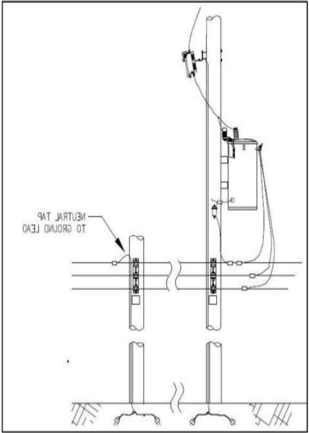
Diagram of good connections on the neutral
