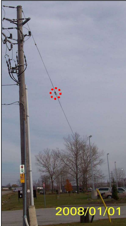
Acceptable Guy Wire and Johnny Ball
