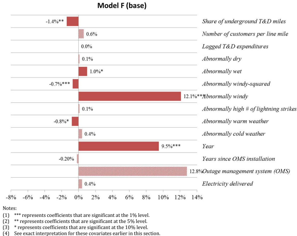
Figure 24: Percentage change in SAIDI (with major events) corresponding to a change in the explanatory variable
