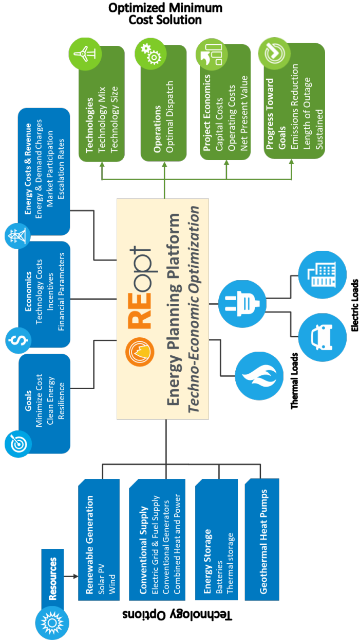
Figure 1. Diagram of REopt’s inputs and outputs
